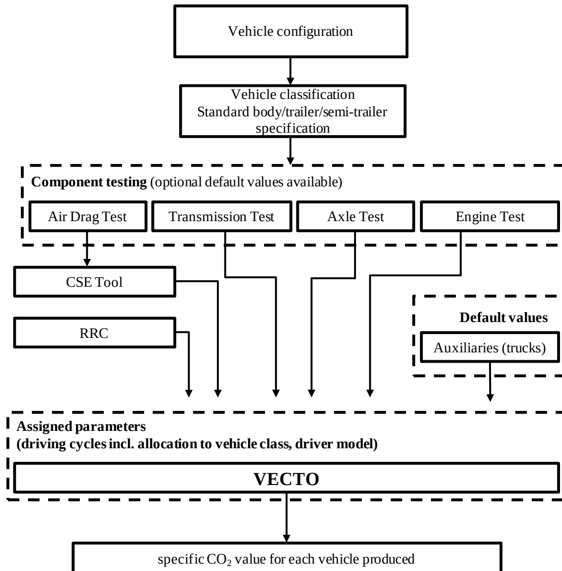
Fig. 3-1: Process scheme
