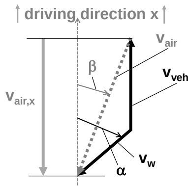
Fig. 5-1: Geometrics of air flow and vehicle speed
