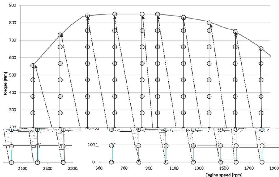
Fig. 5-2: Measurement points for fuel map
