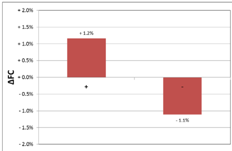
Figure 53: FC change for +/- 0.3 [kg/t] rolling resistance results for 24t 6x2 Coach
