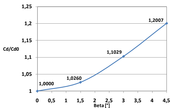
Figure 33: Cross flow drag force coeff. ratio
