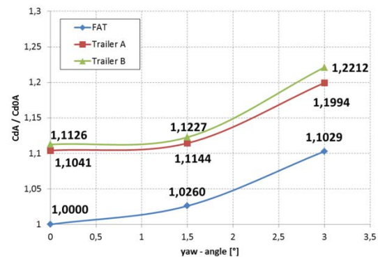
Figure 46: ratio of C_D \cdot A from alternative trailer to standard trailer
