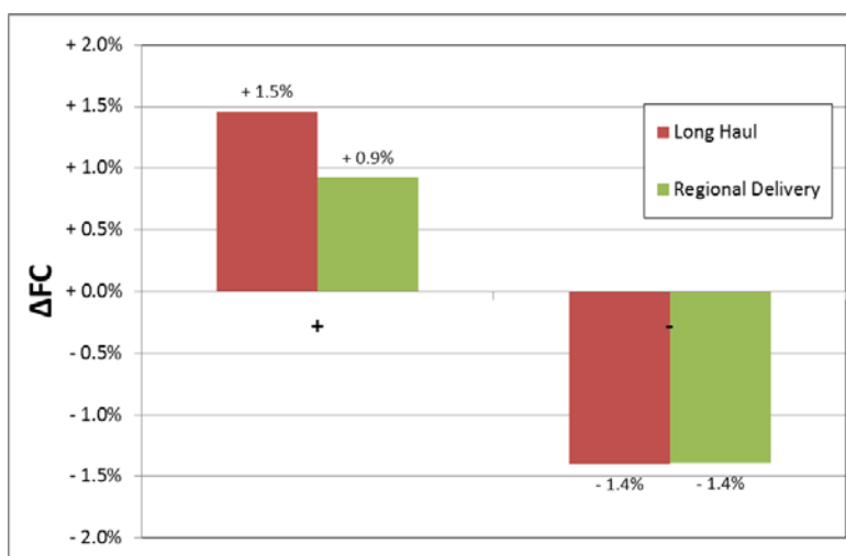
Figure 52: FC change for +/- 0.3 [kg/t] rolling resistance results for 40t 4x2 Tractor & Semi-trailer
