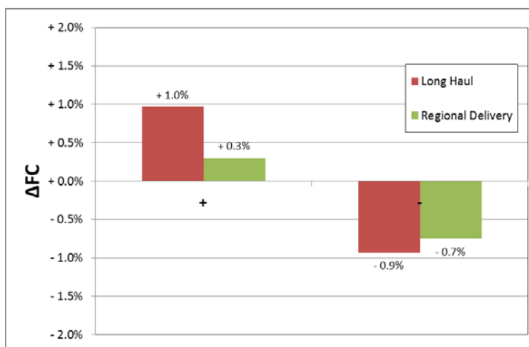
Figure 49: FC change for +/- 3% air drag results for 40t 4x2 Tractor & Semitrailer
