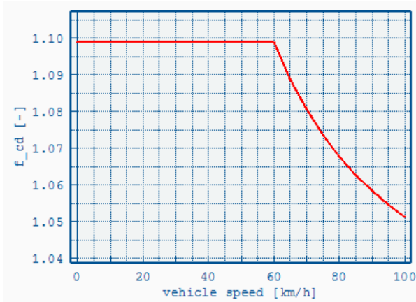
Figure 72: Drag coefficient scaling factor for cross wind correction
