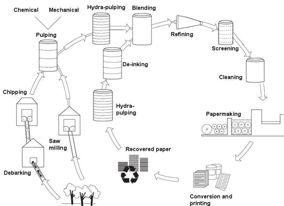
Figure 4.4 Process steps for integrated paper and paperboard production 131
