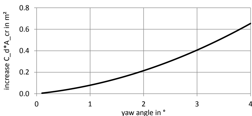
Figure 11: Characteristic curve of the yaw angle effect 11
