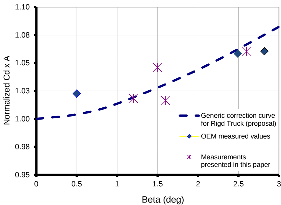
Figure 9 Normalized air drag vs yaw angle results for the CF75. Dashed line corresponds to the curve used for correcting results based on average yaw angle ( \beta ) in the Vaimob+yaw case.
