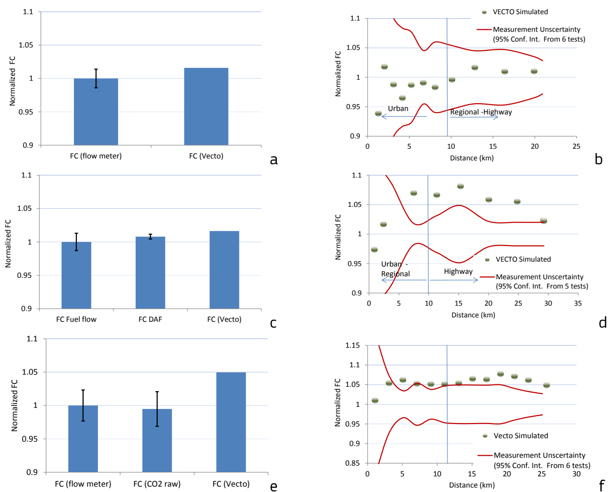
Figure 20 Measured vs simulated results for the driving cycles tested, WHVC (a-b), FIGE (c-d) ACEA regional (e-f). Error bars correspond to \pm -standard deviation of the measurements (sub figs a,c,e) whereas red lines to the 95% confidence interval of the tests
