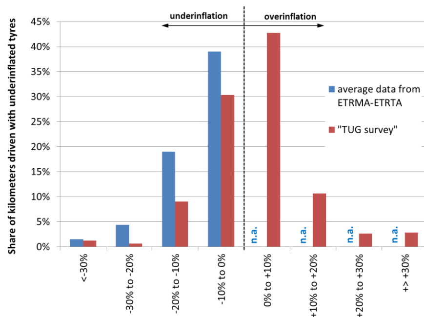
Figure 4: Tyre pressure distribution in the field – "TUG survey"
