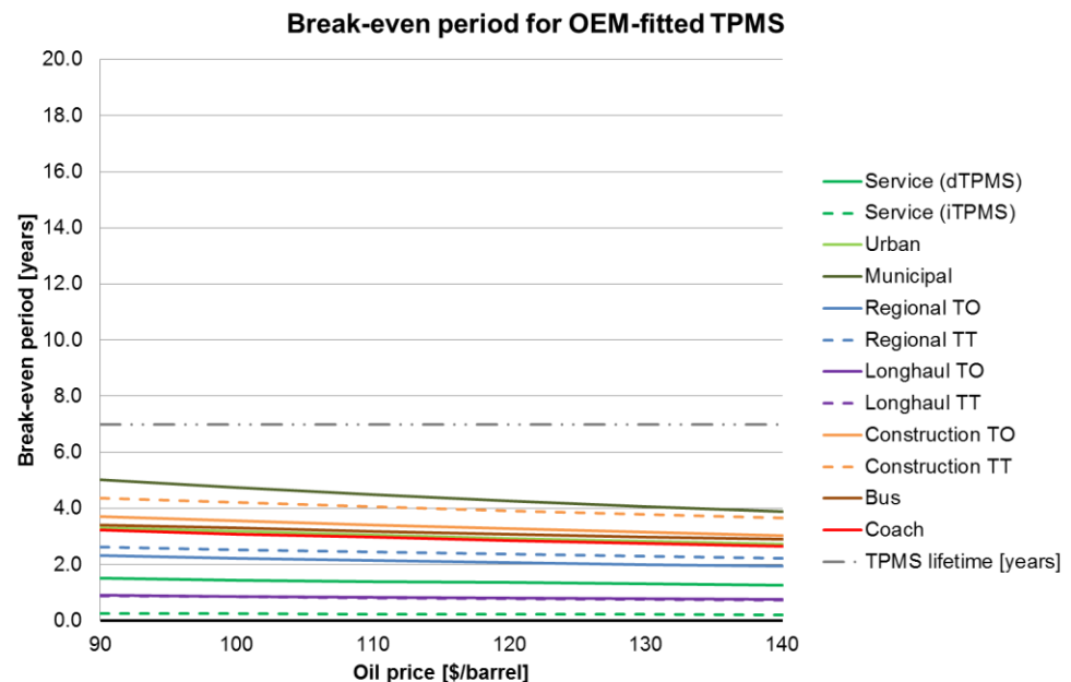
Figure 2: Break-even period for an investment in OEM-fitted TPMS from an end-user perspective , with cost assumptions according to the “ current cost / high savings potential ” scenario and taking account of all relevant cost changes (investment costs, fuel cost savings, and changes in other operation costs).
